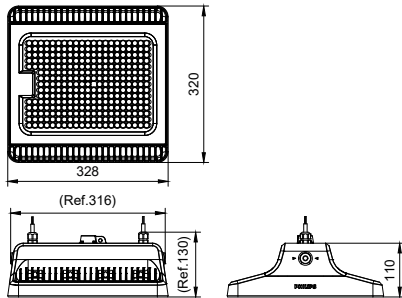
BY570P LED250/865 PSU WB CAU CL
