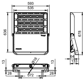
BVP384 LED614/NW 490W 220-240V SMB GM
