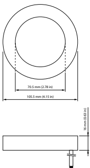
LCU7591 Amplight Leak Coil
