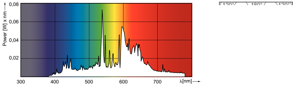
LDPO_CDMR111E_0001-Spectral power distribution Colour
