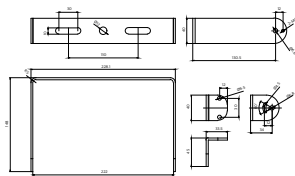
BY240Z Bracket
